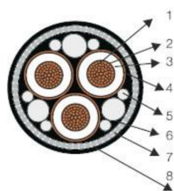
Cross-sectional view
