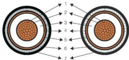
Cross-sectional view
